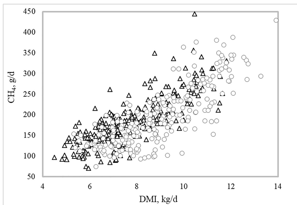
Fig 2. Relationship between enteric methane (CH 4 ) emissions and dry matter intake (DMI) of Nellore bulls and heifers classified as negative (triangle) or positive (circle) residual feed intake (RFI). The general linear regression equation of CH 4 on DMI was: y = 39.0 (\pm 14.6) + 17.5 (\pm 1.23)x + \text{residual} .
