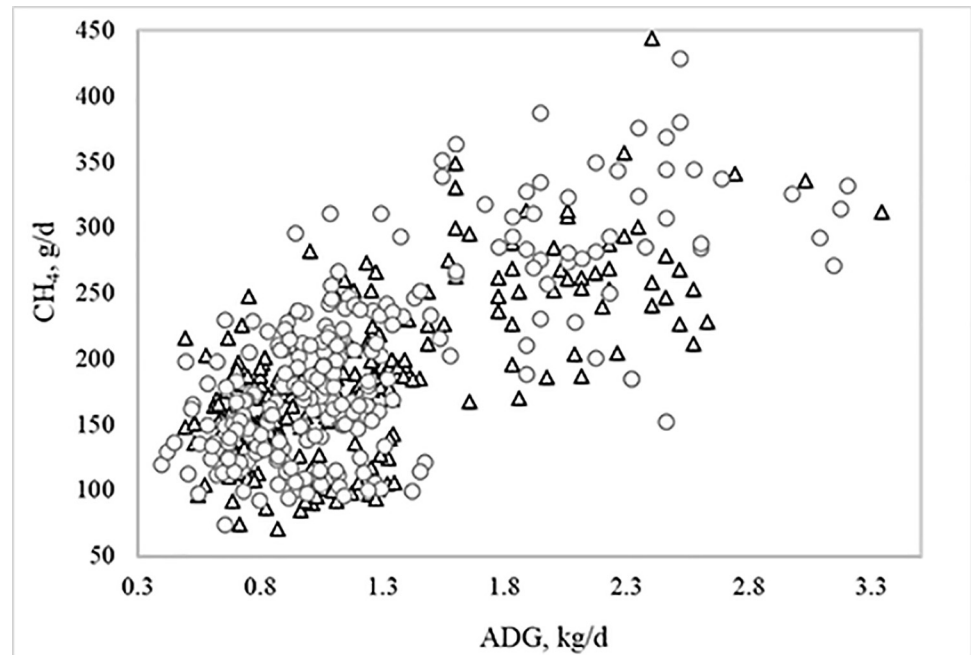
Fig 3. Relationship between enteric methane ( \text{CH}_4 ) emissions and average daily gain (ADG) of Nellore bulls and heifers classified as negative (triangle) or positive (circle) residual feed intake (RFI). The general linear regression equation of \text{CH}_4 on ADG was: y = 112(\pm 13.7) + 58.0(\pm 5.31)x + \text{residual} .
