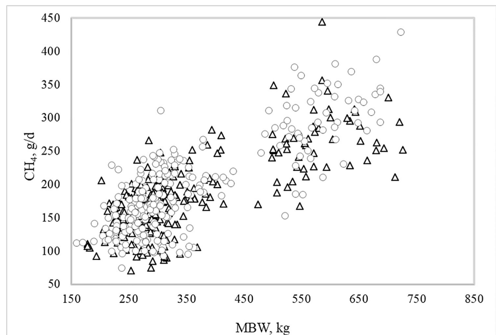
Fig 4. Relationship between enteric methane ( \text{CH}_4 ) emissions and mid-test body weight (MBW) of Nellore bulls and heifers classified as negative (triangle) or positive (circle) residual feed intake (RFI). The general linear regression equation of \text{CH}_4 on MBW was: y = 35.7(\pm 13.9) + 0.43(\pm 0.030)x + \text{residual} .
