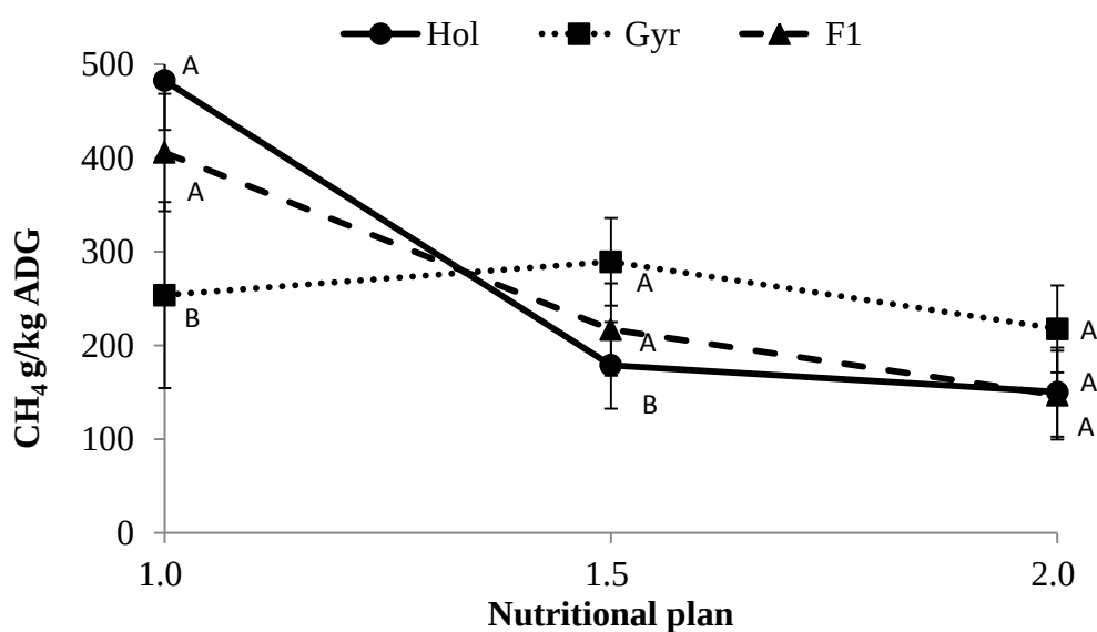
Figure 4 - Effect of interaction between genotype and nutritional plan to \text{CH}_4 g/kg of ADG
